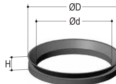
Anel V´ring
