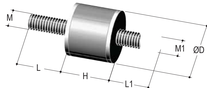
Coxim Macho
