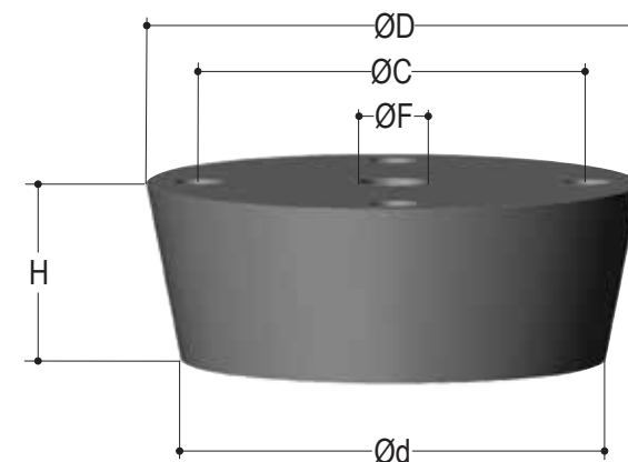
Tampa p/ Moinho c/ Furo Central
