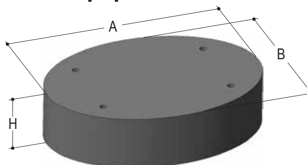
Tampa p/ Moinho Oval
