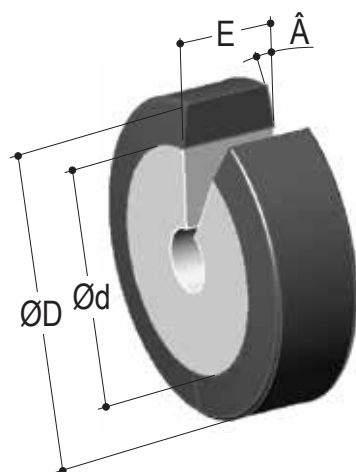
Roldana c/ Chanfro
