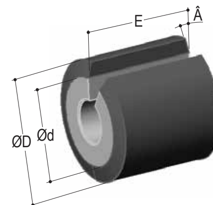
Roda c/ Chanfro
