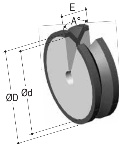
Roldana c/ Chanfro
